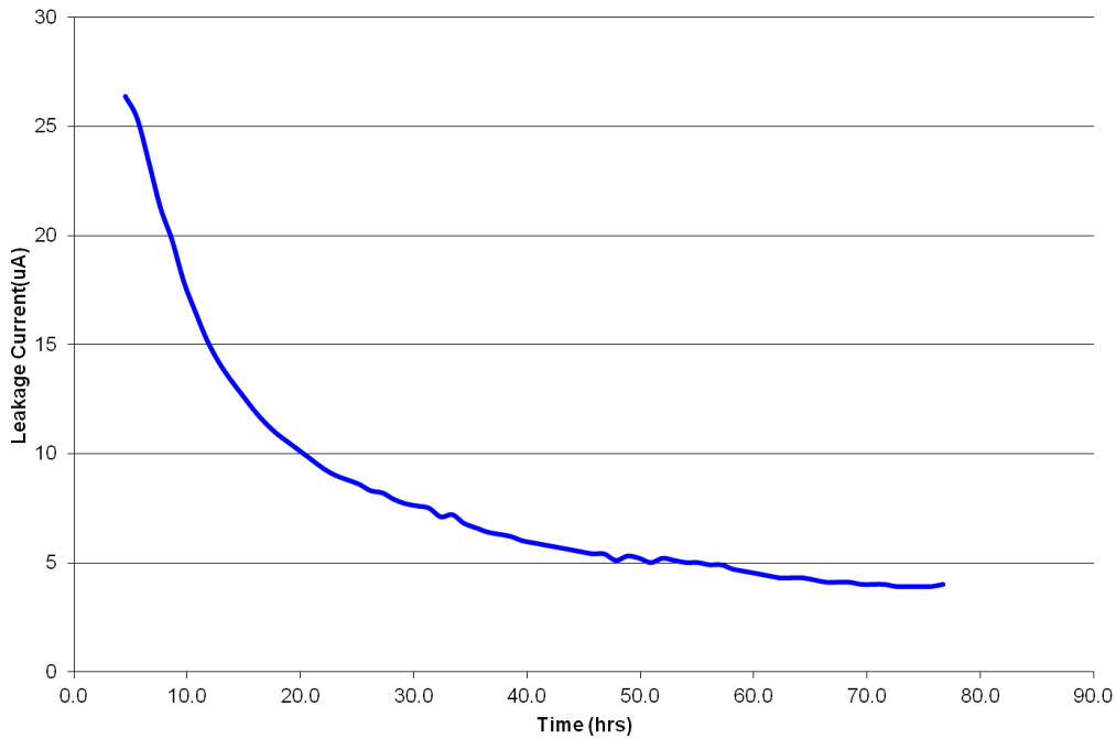
Fig 10: Leakage Current
