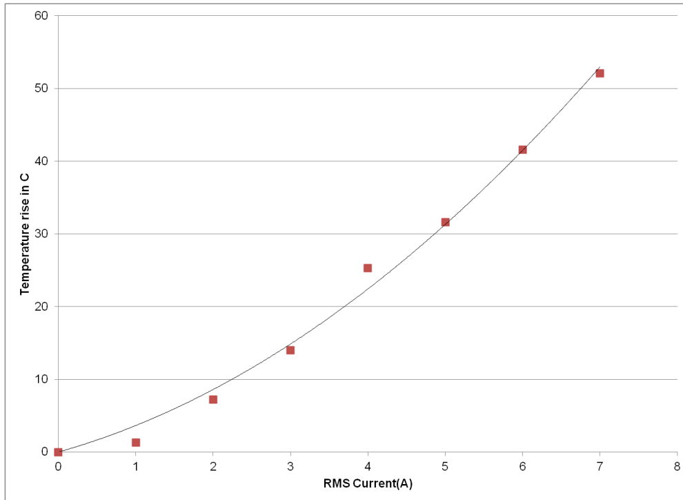
Fig 12: Temperature rise in HS230 with RMS current
