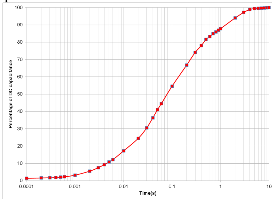
Figure 4: Effective Capacitance
