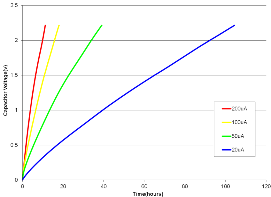
Fig 11: Charging an HS130 with low current
